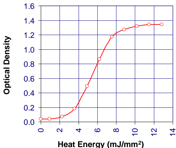
Dynamic Sensitivity
