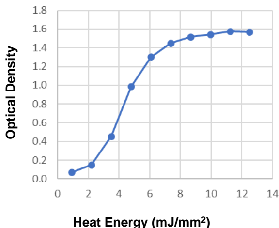
Dynamic Sensitivity
