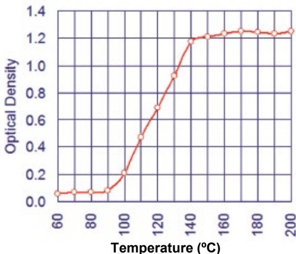
Static Sensitivity
