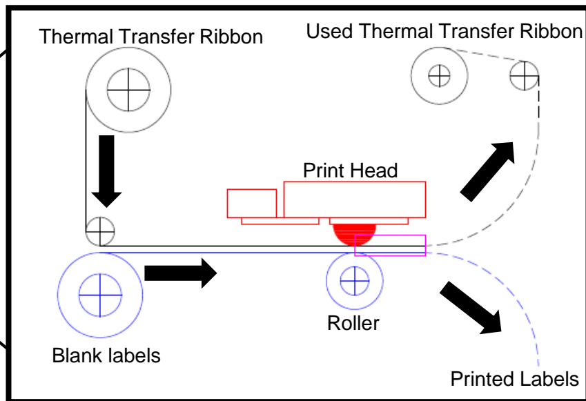
Internal Schematic (varies by printer model)
